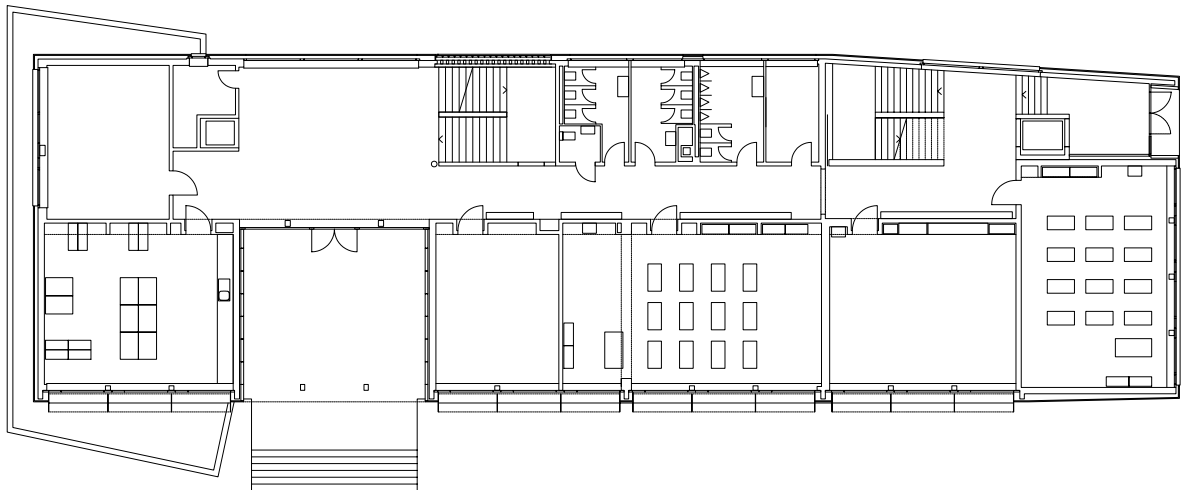
Plan rez - Ecole
