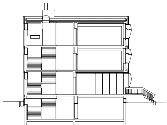
Coupe transevsale - Ecole
