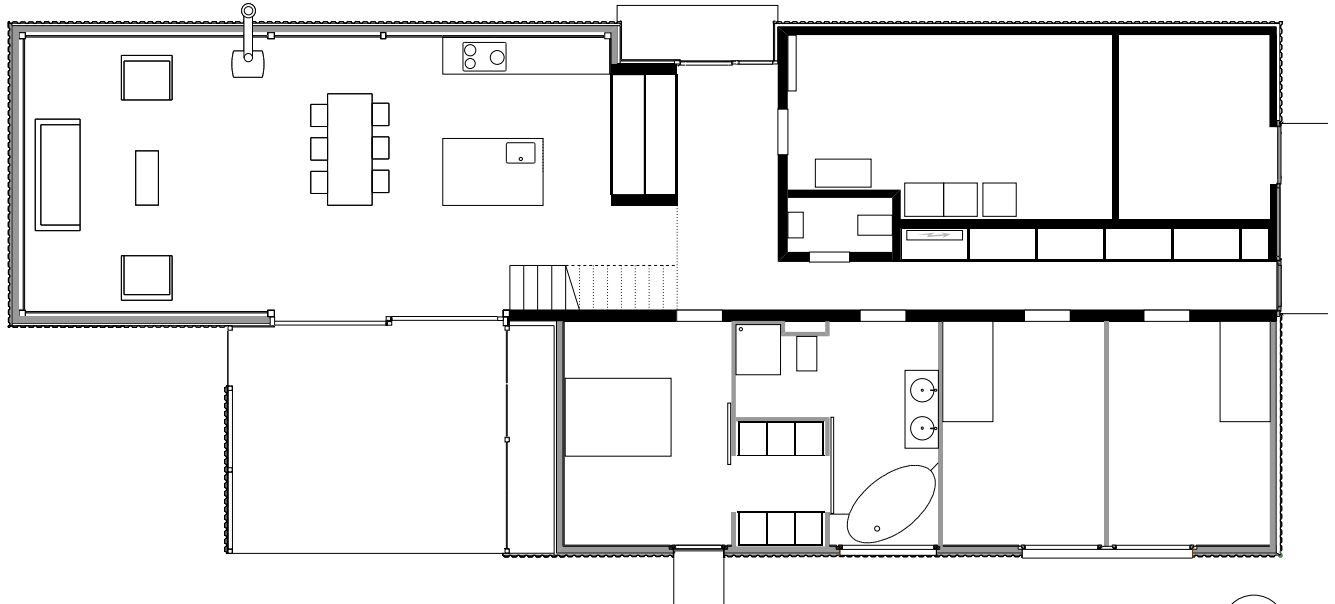
Plan rez
