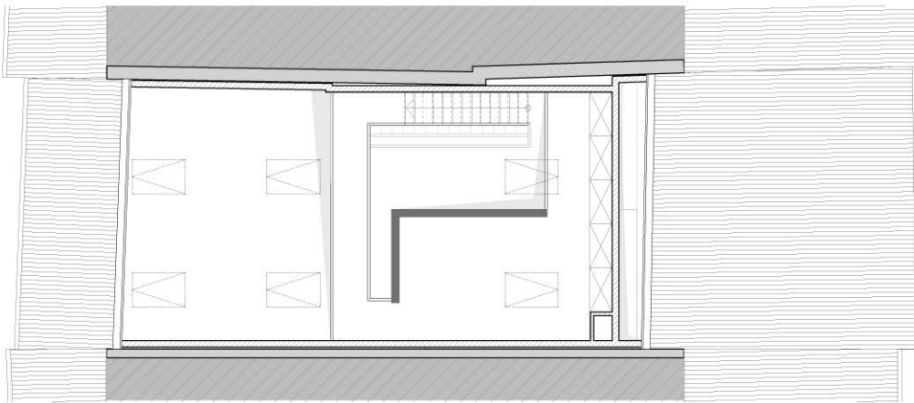
COMBLES
