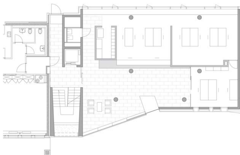
PLAN REZ
