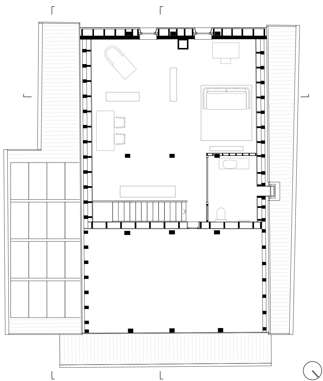
COMBLES
