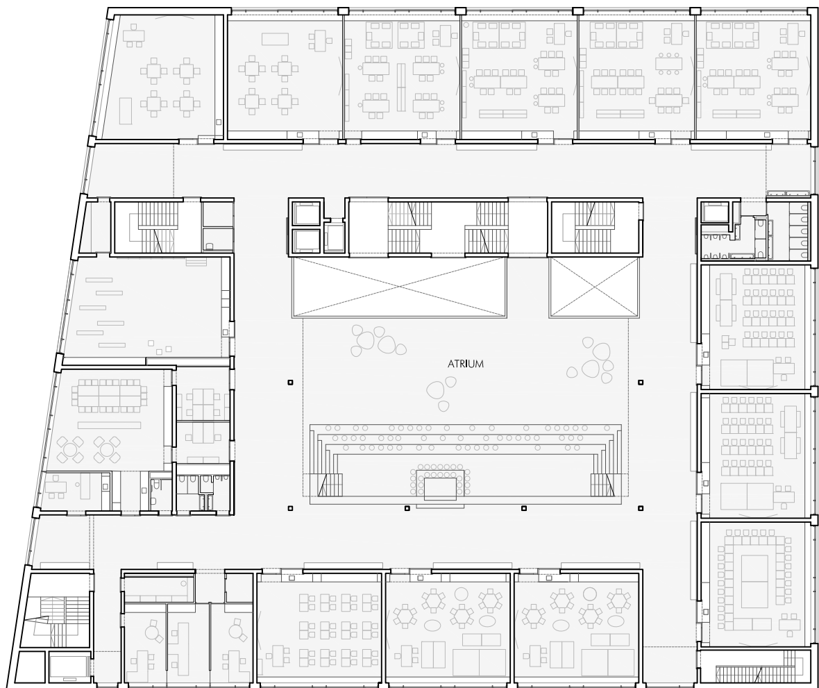
PLAN R+1
