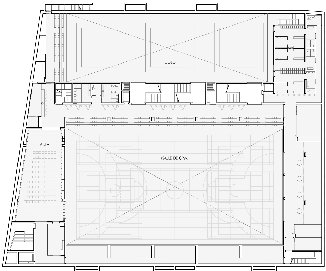
PLAN SS-1
